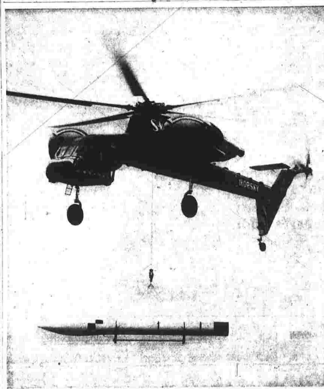
The S-60 crane helicopter rises into the air with a weighted dummy of the Honest John missile. A literal skyhook, the S-60 will give the armed forces unusual mobility in transporting missiles and other heavy equipment.
